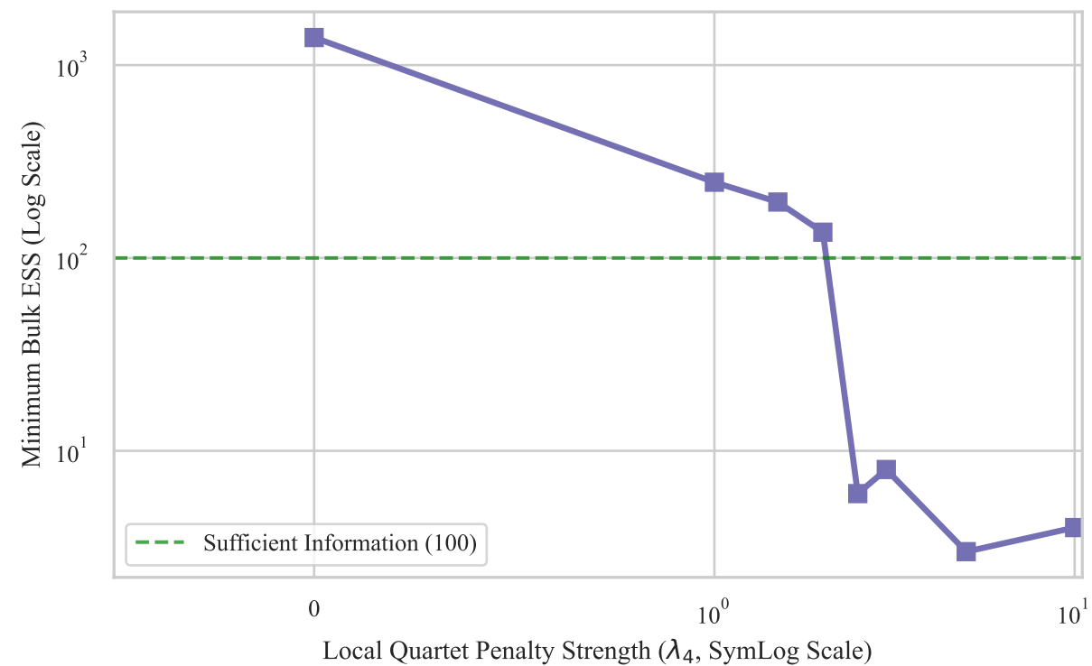
(B) Phase 2 Sample Information Capacity
